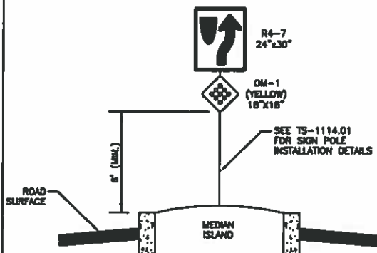
MEDIAN ISLAND DETAIL
